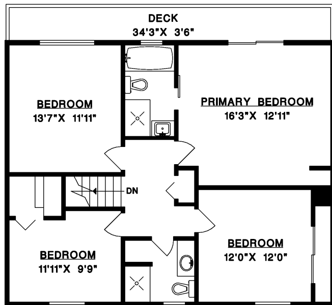
UPPER FLOOR
